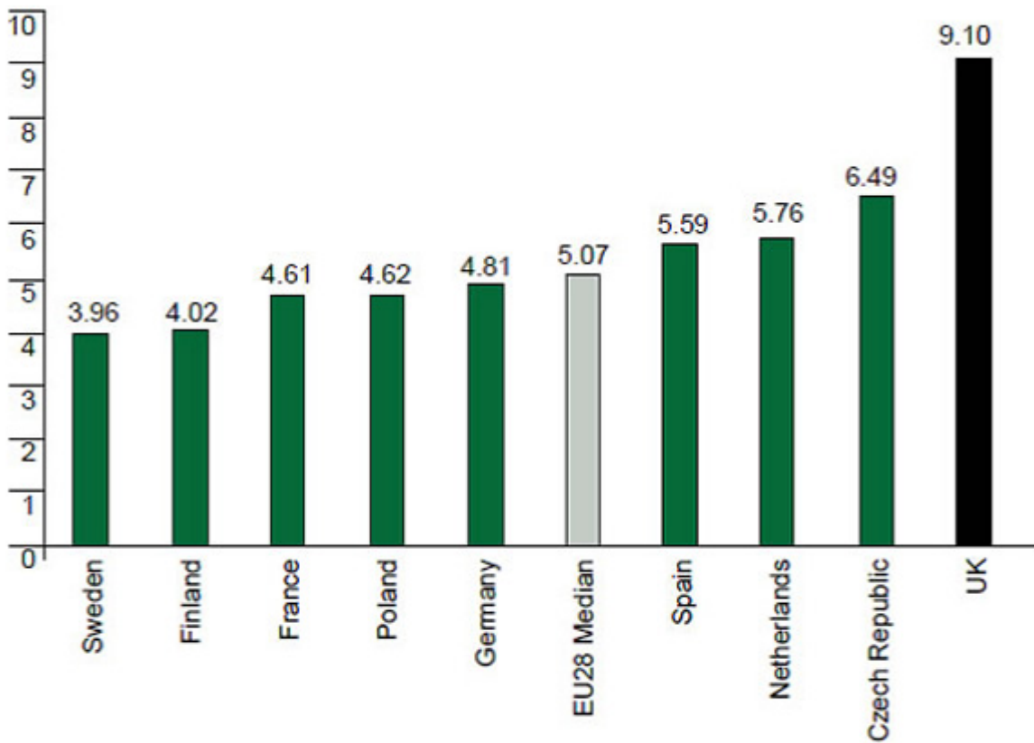
Source: Eurostat / DUKES December 2014
