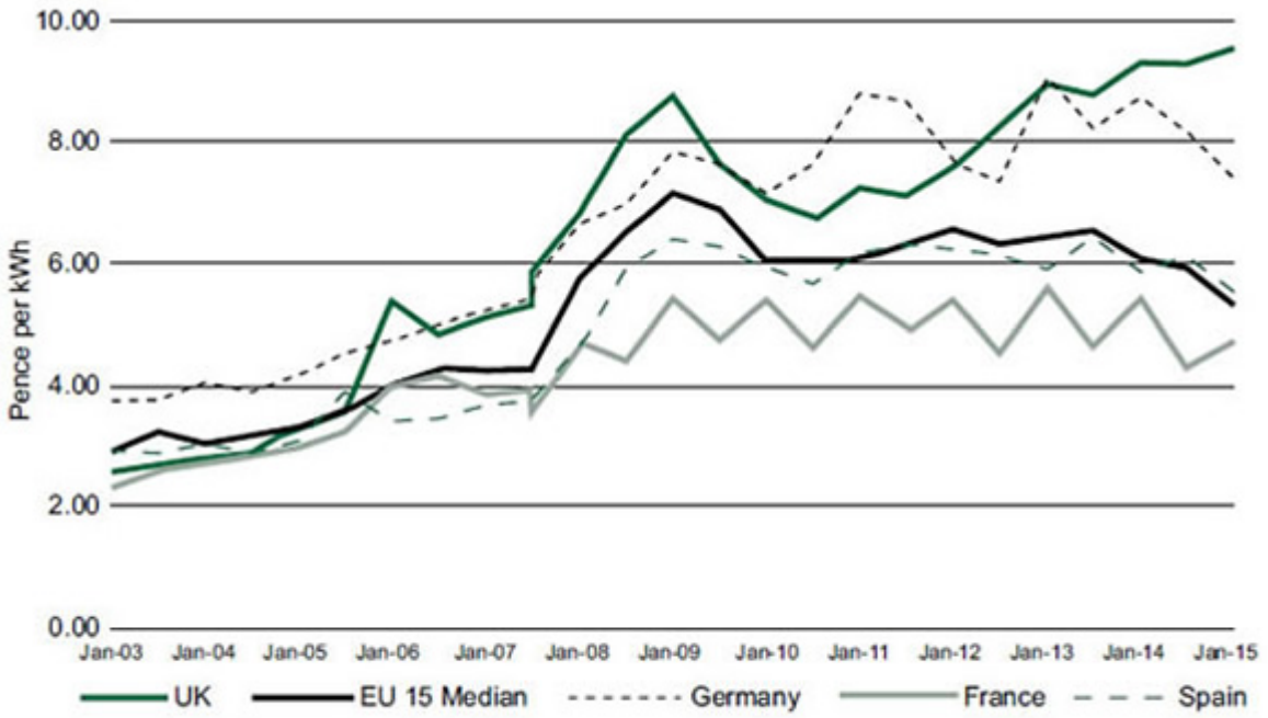
Source: DECC, Statistical data set, International industrial energy prices International price comparisons, Table 5.4.4. Note that the definition of extra large user changed in 2007.
