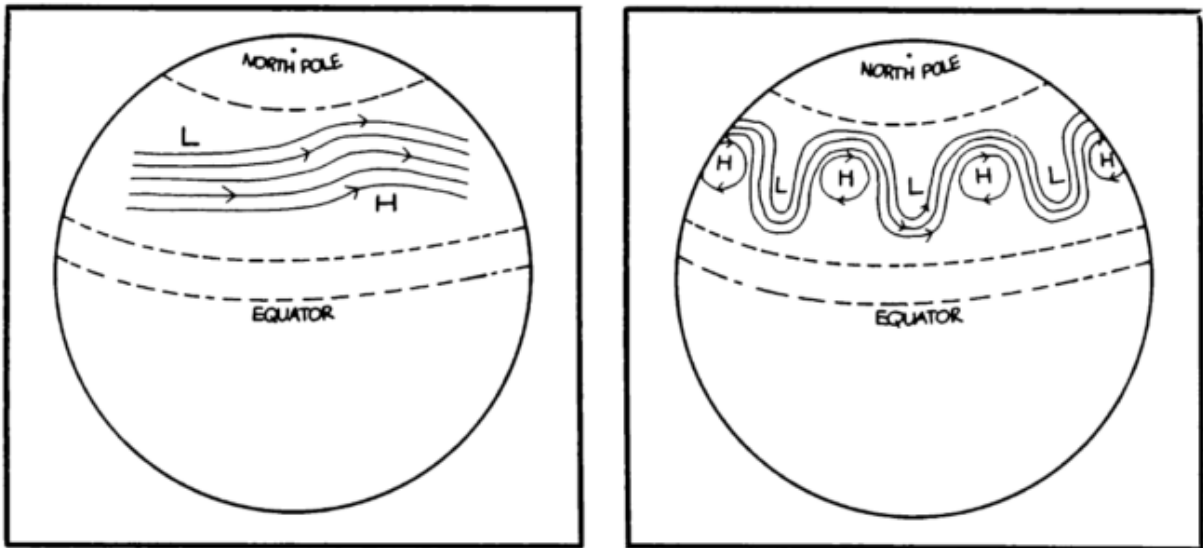
Warm "zonal circulation" winds (left); cool "meridional circulation" (right).
